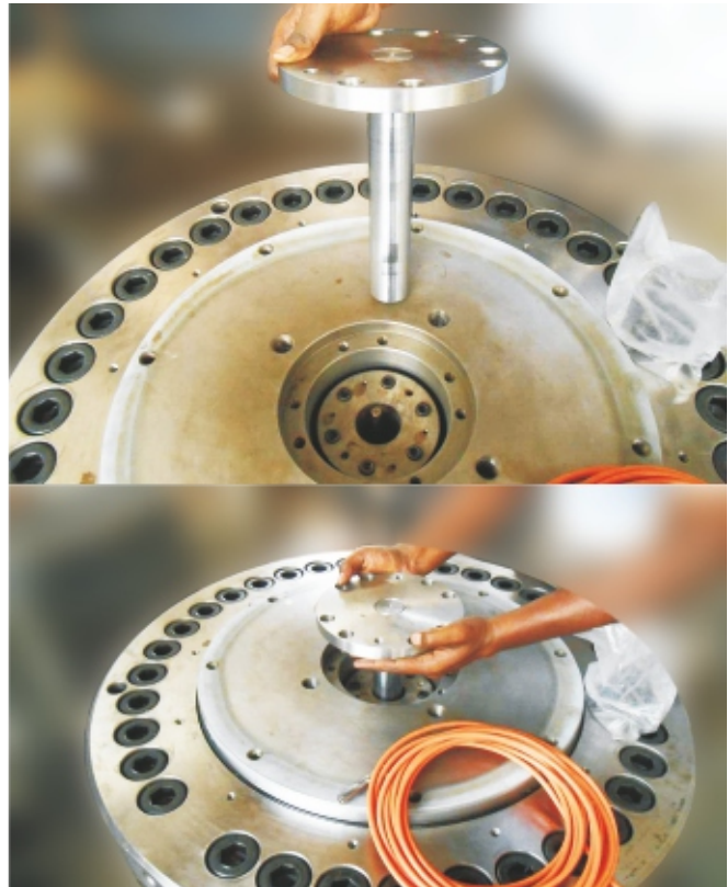
4, 5. Typical Views of fixing internal position transducers (LVDT) in \varnothing 600mm Roll Force Cylinders
