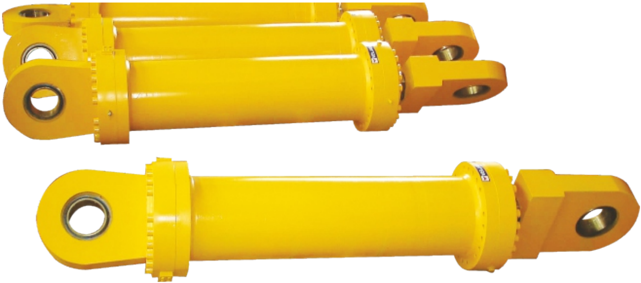
8. Typical View of packing of bore 360mm \varnothing x 200mm Piston Rod x 1500mm Stroke Stacker Reclaimer Hydraulic Cylinders (Operating Pressure 250 Bar Test Pressure 375 bar)
