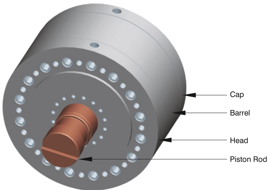
Fig.4 Hydraulic Rotary Cylinder Bore \varnothing 600mm x Piston Rod \varnothing 560mm x Stroke 65mm.
