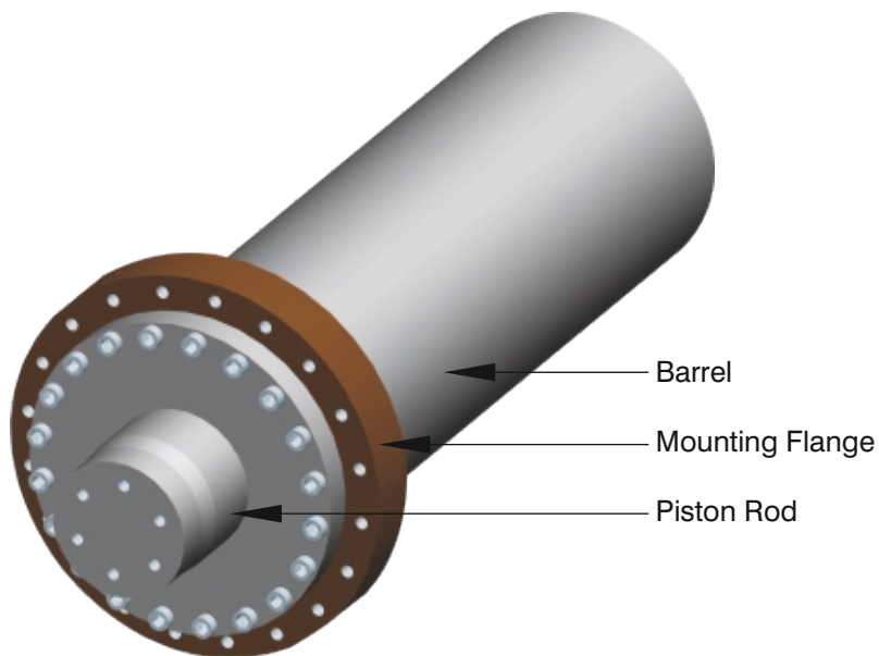
Fig.3 Heavy Duty Hydraulic Cylinder Bore \varnothing 450mm x Piston Rod \varnothing 300mm x Stroke 1250 mm. Working pressure at 300 bar & Test pressure 450 bar.
